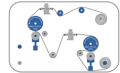
Double side printing route
